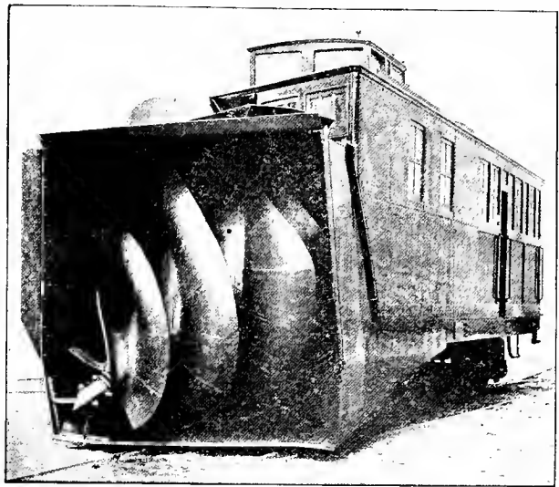
Fig. 226. THE JULL CENTRIFUGAL SNOW EXCAVATOR.
